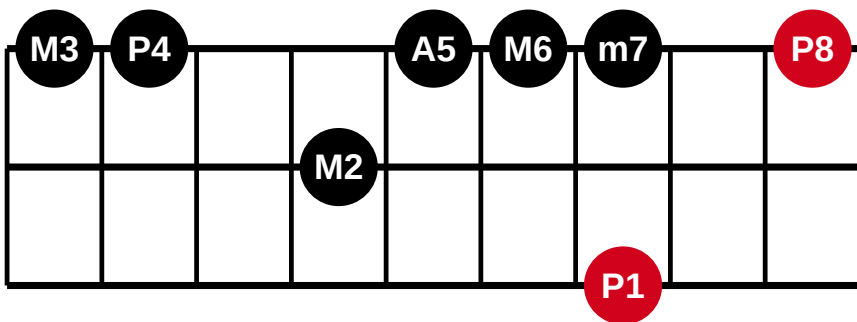
3 strings - 9 frets - fingering 20 of 21
