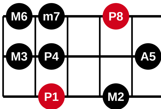
3 strings - 5 frets - fingering 2 of 21
